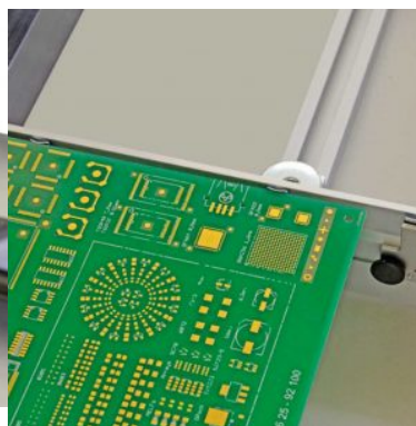
Supporti PCB
